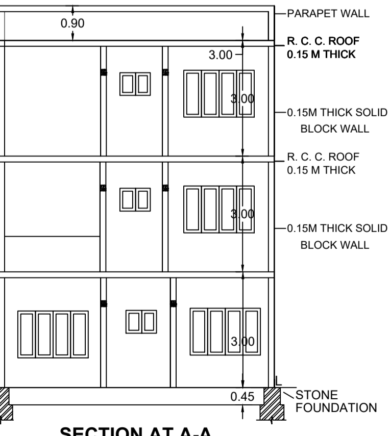
SECTION AT A-A
